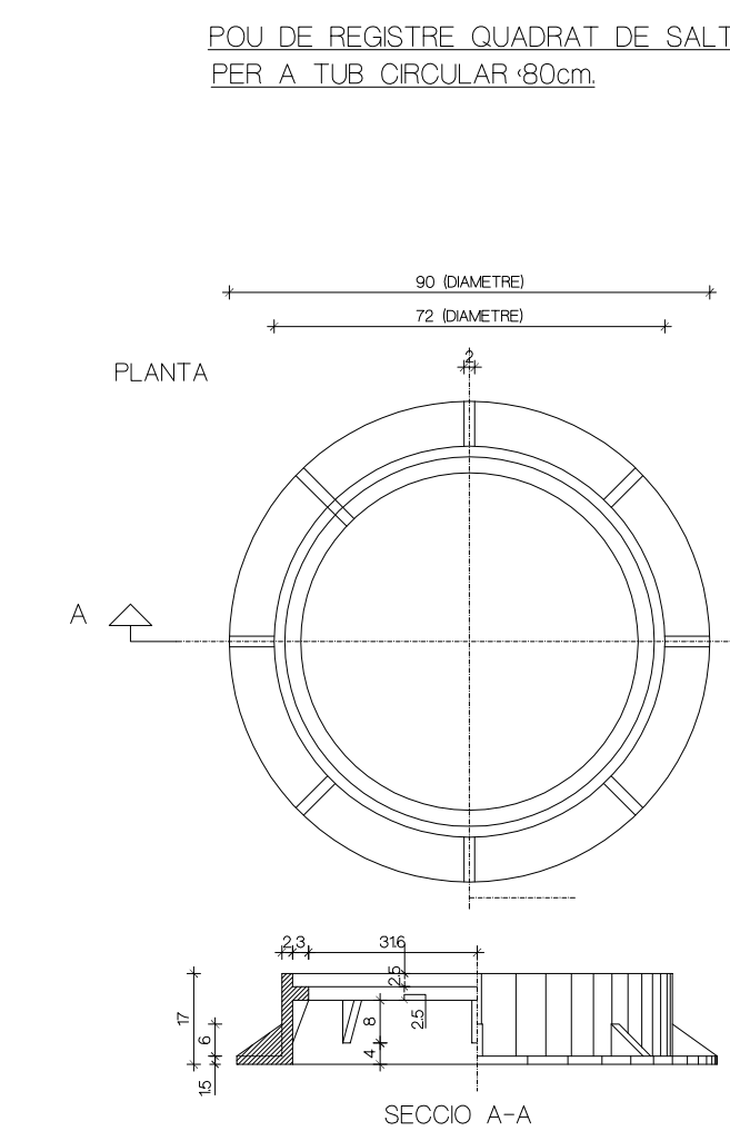
DETALLS CLAVEGUERAM
